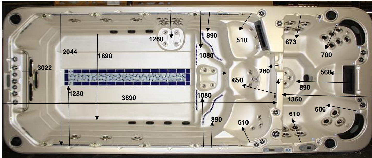
Marathon 18/5 Dimensions
